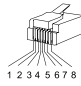
8-pin RJ45 Connector (8P8C)
